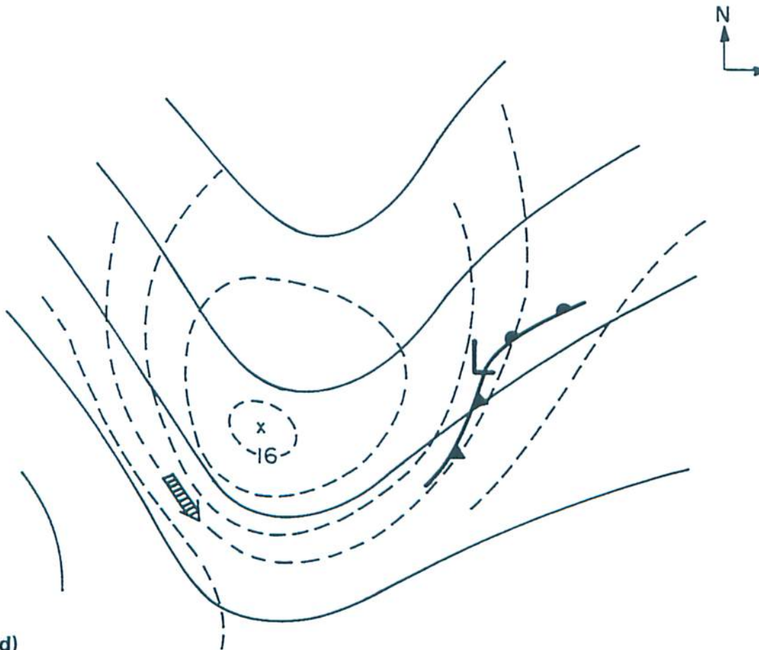
Figure 10.4 (c) Same convention as in (a) except for stage 2 (open wave stage) cyclone development. (d) Same convention as in (b) except for stage 2 in cyclone development.
