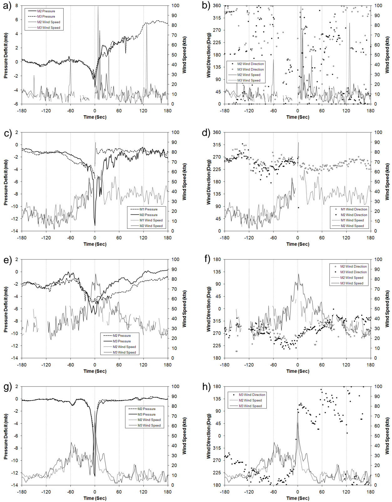
Figure 5. Pressure deficit (mb) and wind speed (kts) versus time for a) May 10 th , c) May 23 rd , e) May 29 th case 1, and g) May 29 th case 2, and wind direction (deg) and wind speed (kts) versus time for b) May 10 th , d) May 23 rd , f) May 29 th case 1, and h) May 29 th case 2. Figures are normalized to the time of vortex passage (0 sec).
