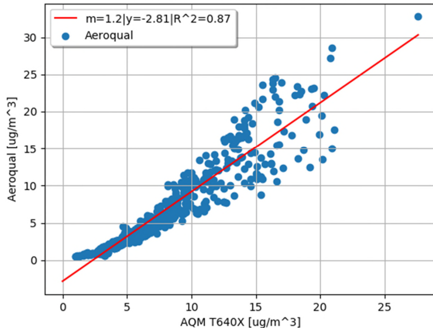
Aeroqual vs T640X (hourly avg.)
